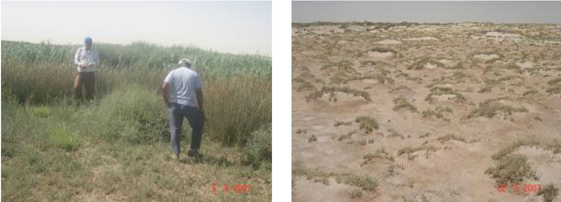
Figure 3: Different types of salt tolerant vegetation (halophyte) at Al Asfar area.
