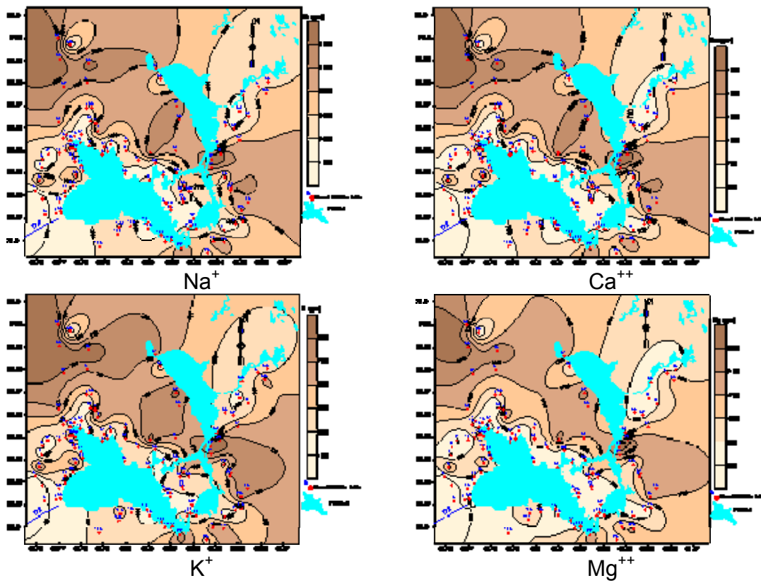
Figure 10, a: Distribution maps of the major cations concentration for the soil of Al Asfar area, Al Hassa, KSA.
