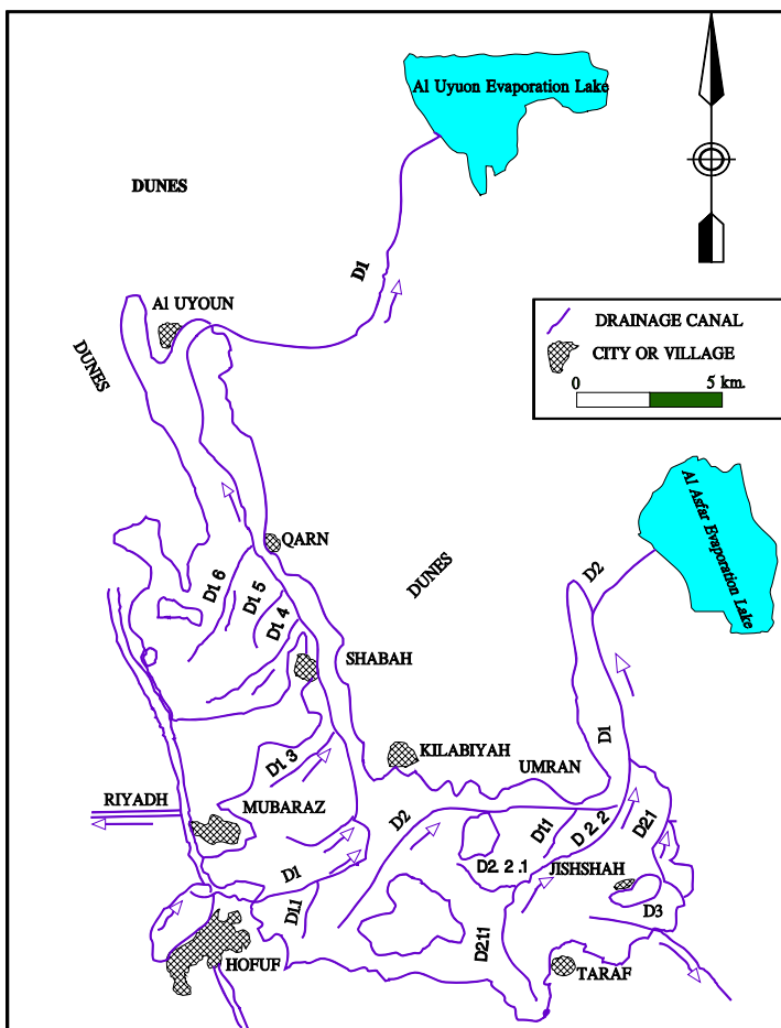
Figure 2: Main Drainage System of Al Hasa Irrigation and Drainage Project.
