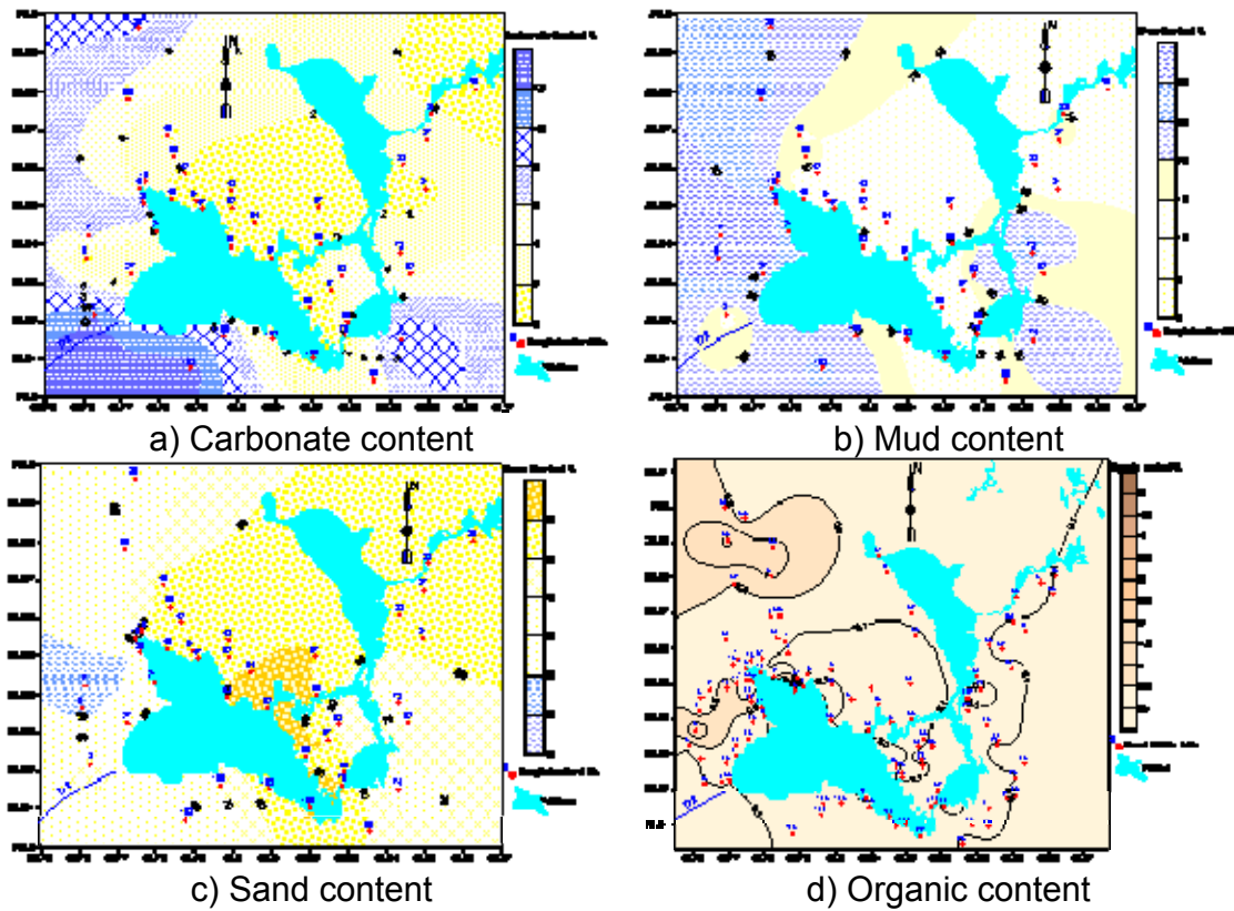
Figure 7: The spatial distribution of carbonate, sand, mud and organic matter contents in the inland sabkha samples of Al Asfar area, Al Hassa, KSA.
