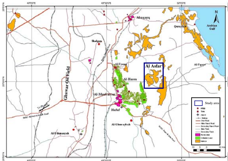
Figure 1: Base map of Al Hasa Region and the location of the study area.
