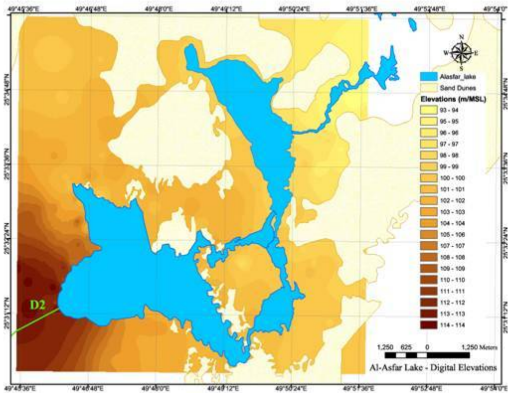
Figure 4: Digital Elevation Model Map of Al Asfar area, Al Hassa, KSA.
