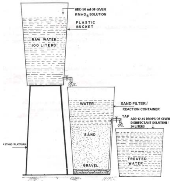
Fig. 1: Portable Instant Water Filter “NEERI-ZAR
