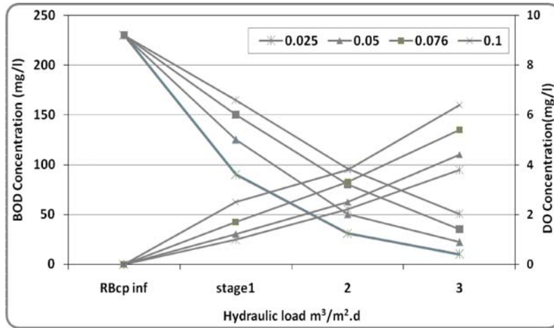
Fig. 5: Effluent DO and BOD concentration from stages in different hydraulic load
