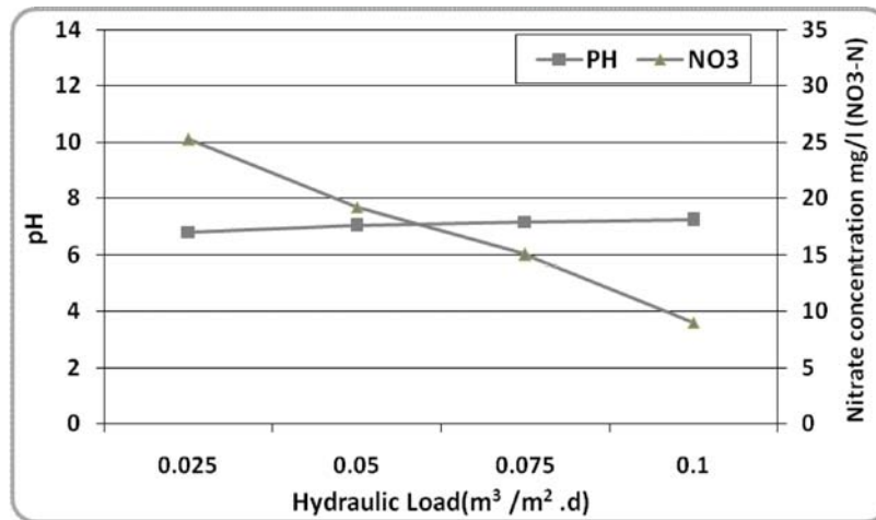
Fig. 7: Effluent pH and nitrate concentration in different hydraulic load
