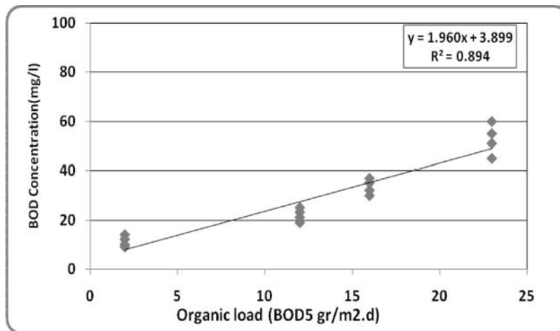
Fig. 9: Relationship between effluent BOD concentration and organic load
