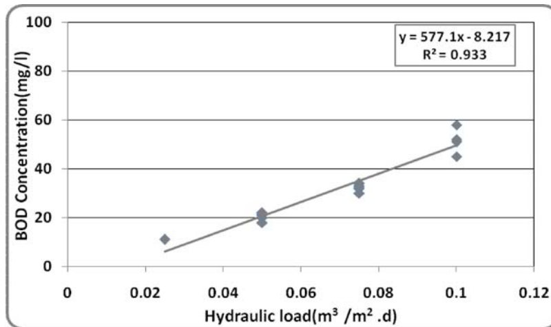
Fig. 8: Relationship between effluent BOD concentration and Hydraulic load
