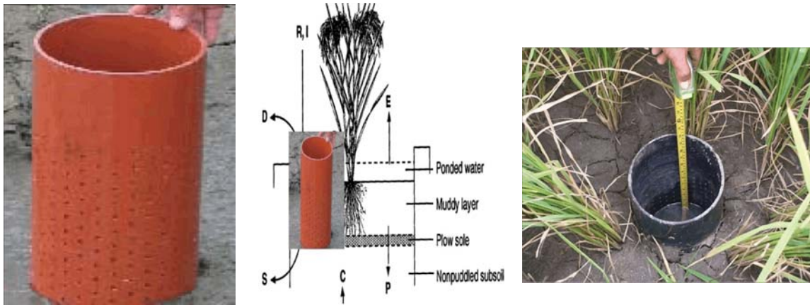
Fig. 1: A simple perforated pipe (water tube) installed in the rice field allows farmer to monitor water level beneath the soil surface
