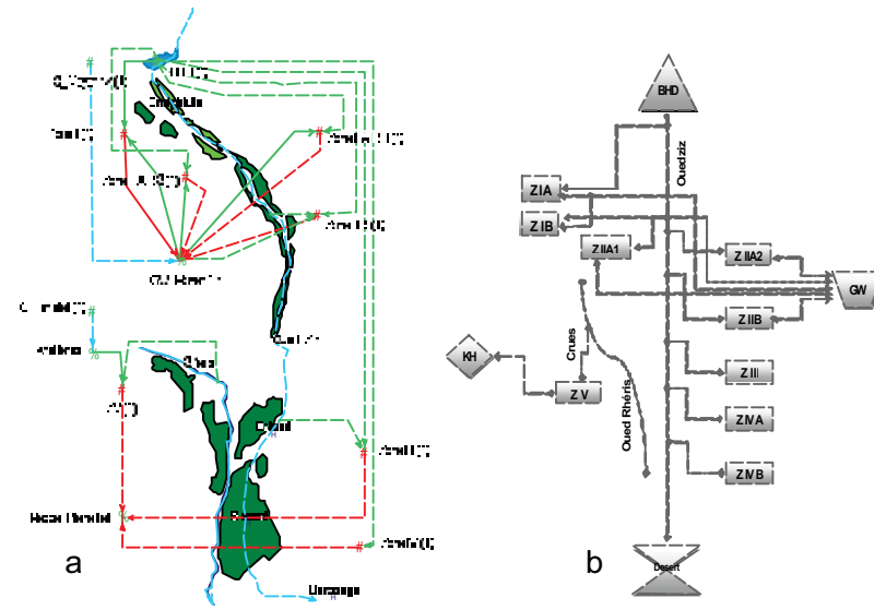
Fig. 4: a) WEAP conceptual Model for water management and irrigated area in Tafilalet, b) Water distribution in main parts of the Ziz oasis BHD: Barrage Hassan Addakhil; KH: Khetaras; Z: Zone, GW: Groundwater
