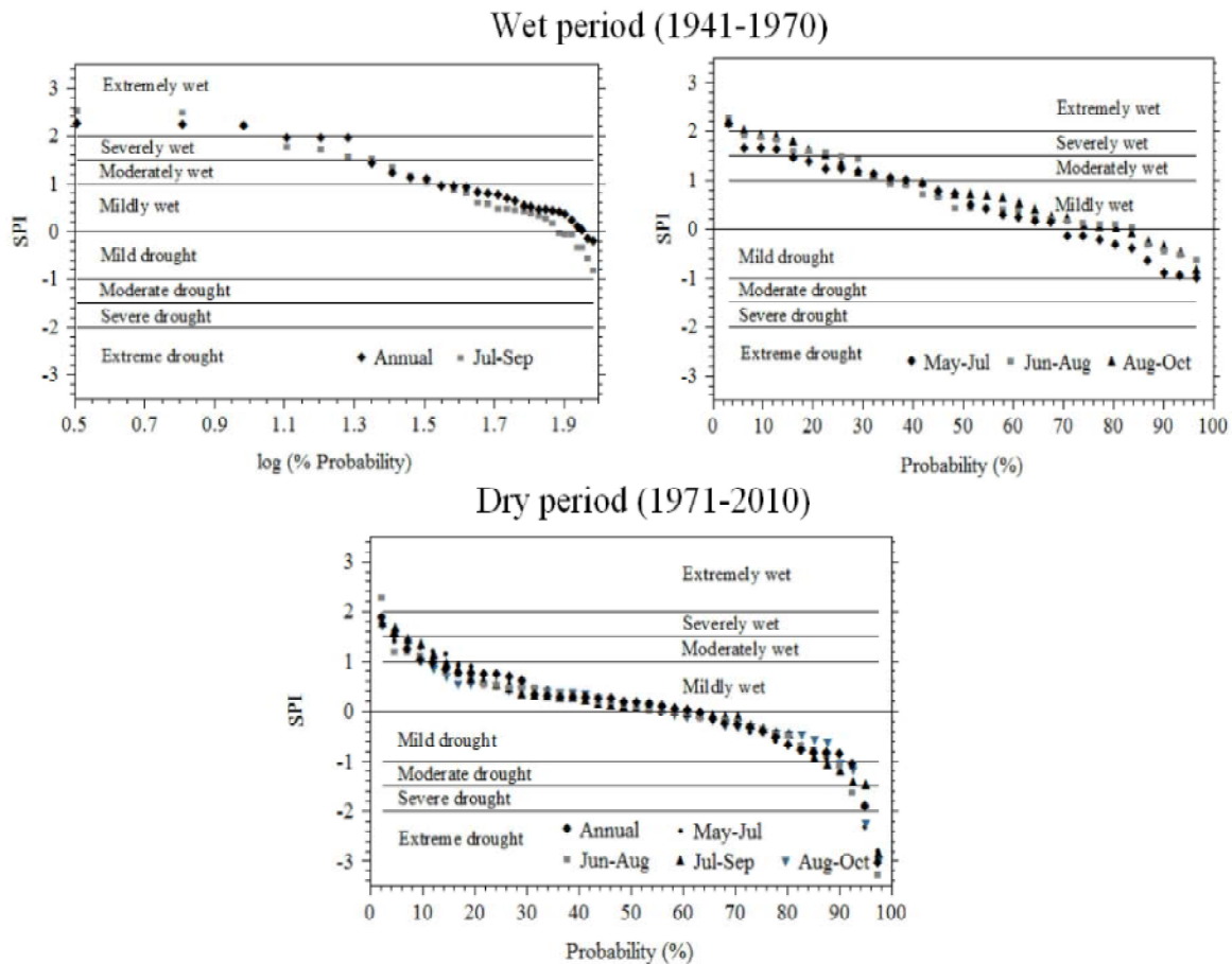
Fig. 3: Scatter plot of SPI probability curves for the wet and dry periods
