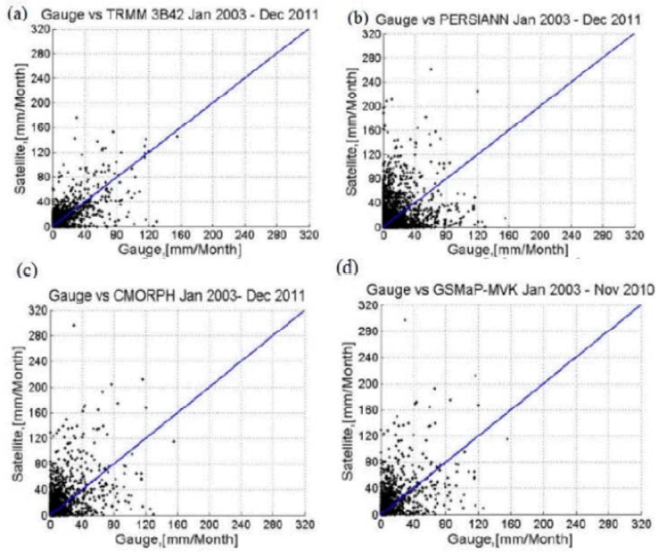
Fig. 8: Scatter plot rainfall estimates over Saudi Arabia at monthly time scale and 0.25° long/ lat special resolution of four different satellite products.
