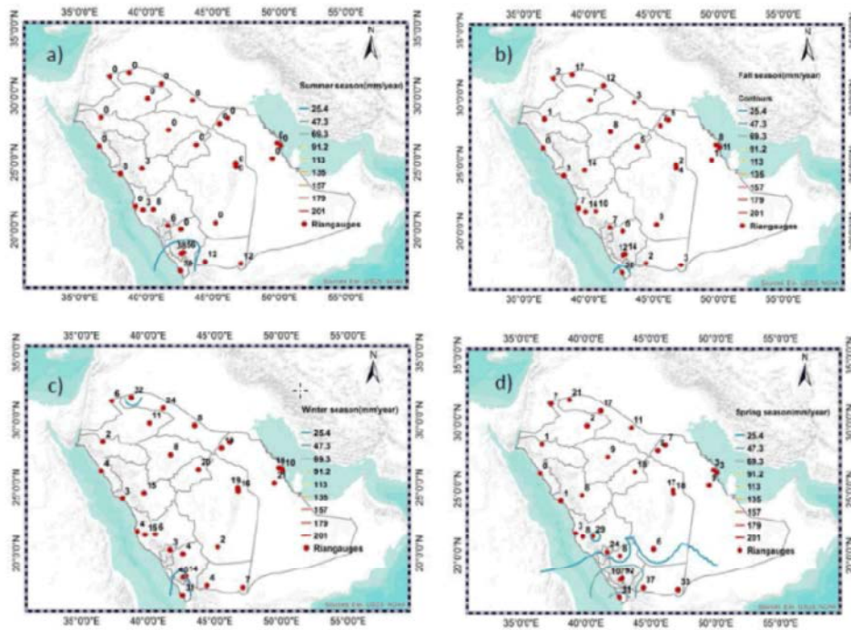
Fig. 5: Average annual precipitation isohyetal contour lines over Saudi Arabia in (a) the summer, (b) the autumn, (c) the winter, and (d) spring season.
