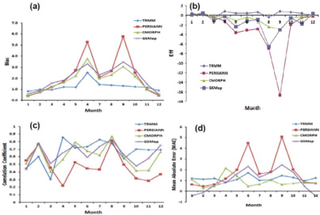
Fig. 7: Monthly validation statistics of (a) Bias, (b) Efficiency, (c) Correlation Coefficient, and (d) Mean Absolute Error of the four satellite products over the region.
