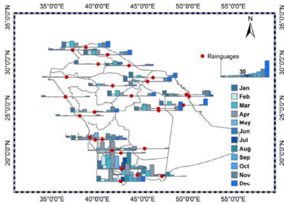
Fig. 2: The average monthly precipitation events from 1985-2005 over the major cities in Saudi Arabia.
