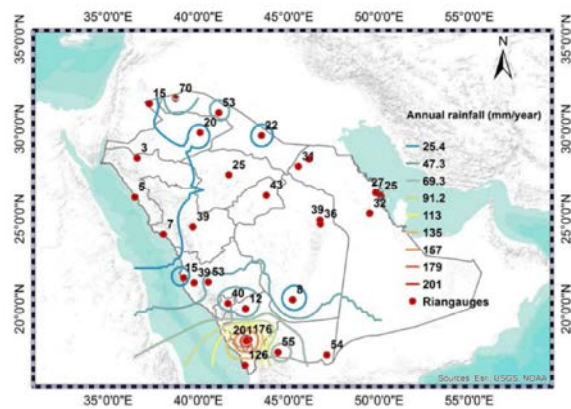
Fig. 4: Average annual precipitation represented in isohyet contour lines for rain gauges over Saudi Arabia.
