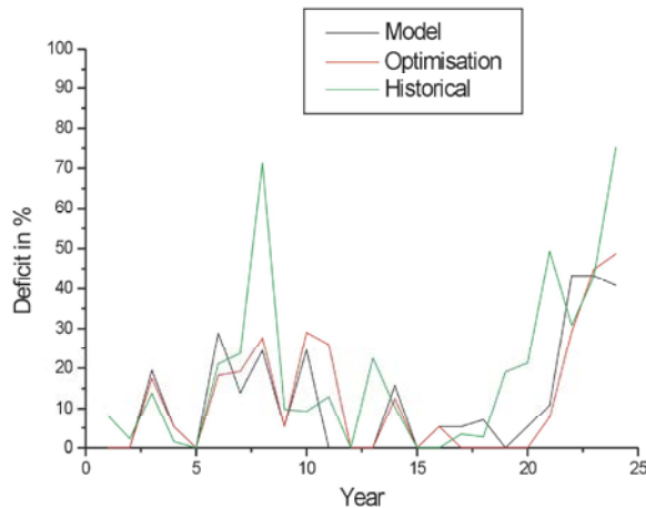
Fig 6: Deficits in % of the second crop for 24 years for different models
