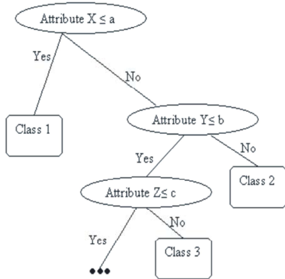
Fig 2: Decision tree abstraction showing how the values associated with certain features determine the class label.
