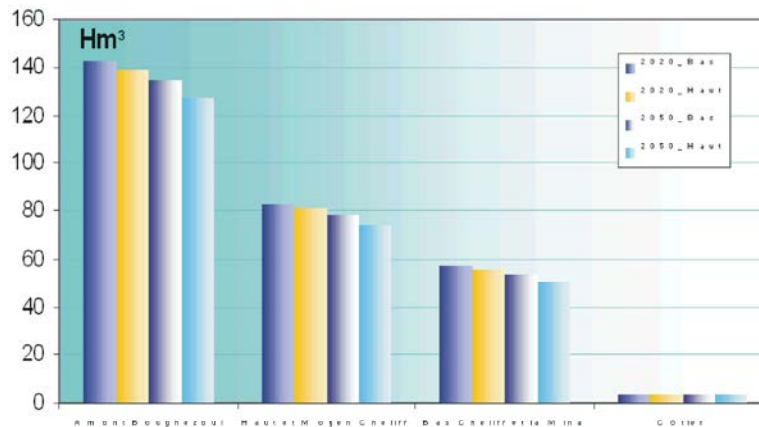
Fig. 2: Distribution of groundwater potential in the Cheliff basin (2020 and 2050).
