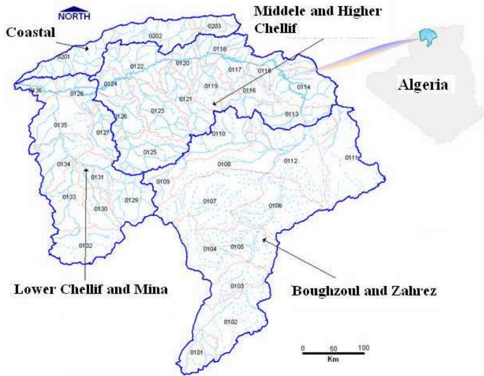
Fig. 1: Studied basins.
