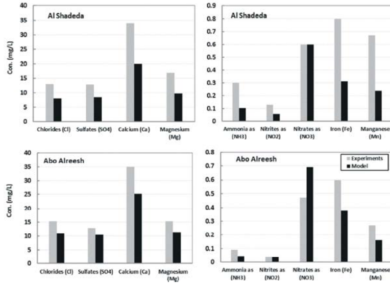
Fig. 8: The modelling results of different constituents in winter time at Al Shadedda and Abo Alreesh stations by Equation 4.
