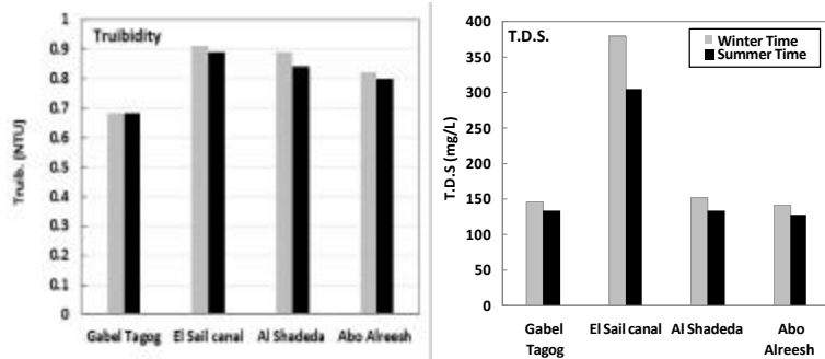
Fig. 2: Average values of turbidity and total dissolved solid for the four suggested positions in winter and summer times
