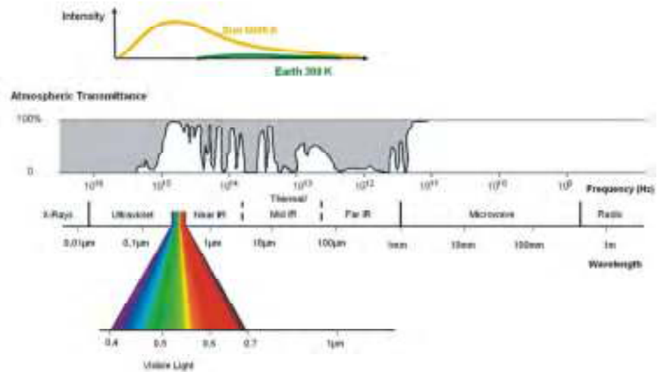
Fig. 4: Electromagnetic Spectrum [4]
