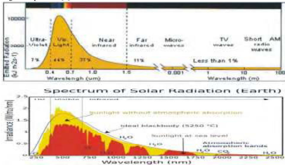
Fig. 4: Electromagnetic Spectrum [4]
