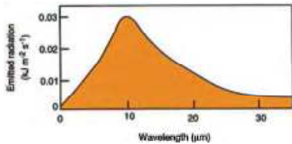
Fig. 6: The Earth Radiation
