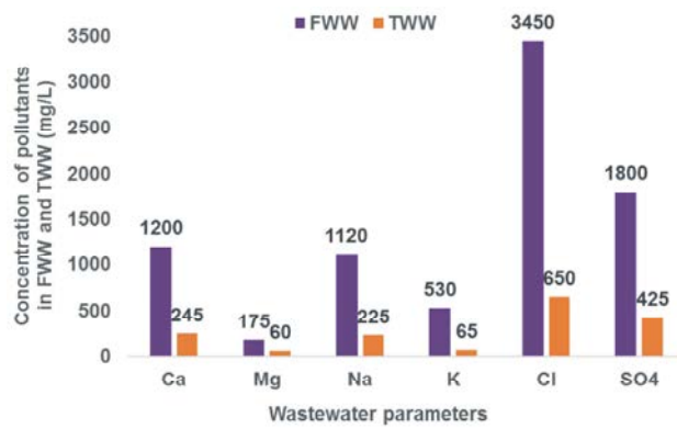
Fig. 4: Level of common metals, chloride and sulphate in feed and treated wastewater
