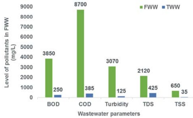
Fig. 3: Characteristics of feed and treated wastewater
