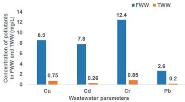
Fig. 5: Level of heavy metals in feed and treated wastewater
