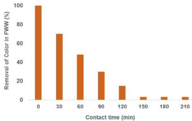
Fig. 6: Removal of color from distillery wastewater
